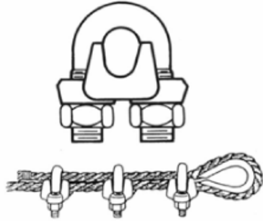
RIGHT WAY FOR MAXIMUM ROPE STRENGTH
